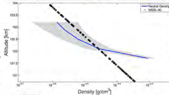
Neutral Density derived from Radar-Detected Meteoroids
